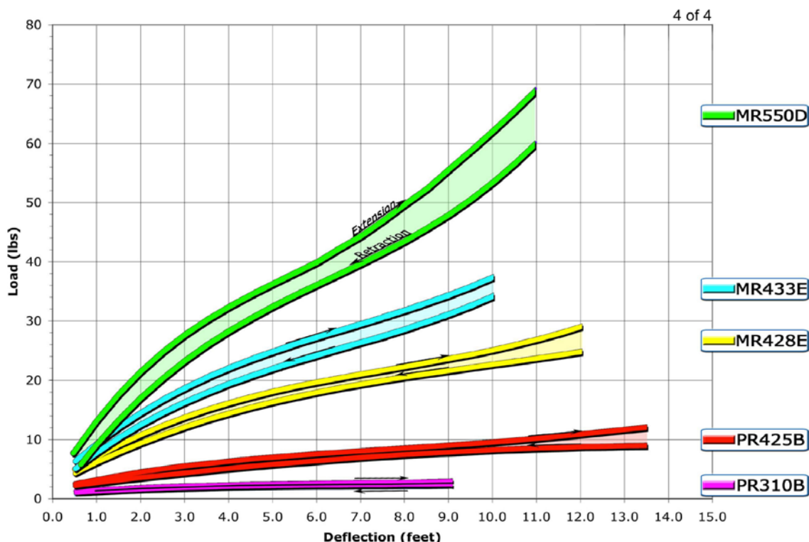
Load vs. Deflection Performance Chart
